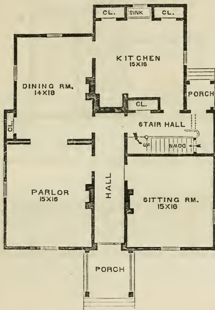
FIRST FLOOR-PLAN.
